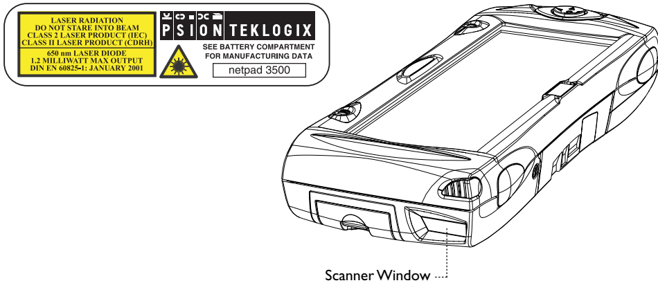
Figure 2.3 Scanner Location
